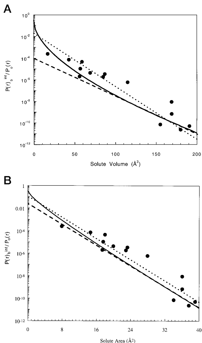
FIGURE 3 ( A ) Comparison of the predicted size dependence of the relative permeability of several solutes across unilamellar egg PC liposomes as a function of solute volume ( solid line ) with the experimentally measured values ( filled circles , see Table 1). The model parameters used for the predictions are discussed in Estimation of Model Parameters. The dashed line corresponds to the trend defined by the large solutes. The dotted line corresponds to a single exponential fit relating relative solute permeability to solute volume. ( B ) Replot of the experimental data and theoretical predictions shown in ( A ) as a function of solute cross-sectional area. The solid line shows the predictions of Eq. 31. The dashed line corresponds to the trend defined by the large solutes. The dotted line corresponds to a single exponential fit relating relative solute permeability to solute cross-sectional area.
