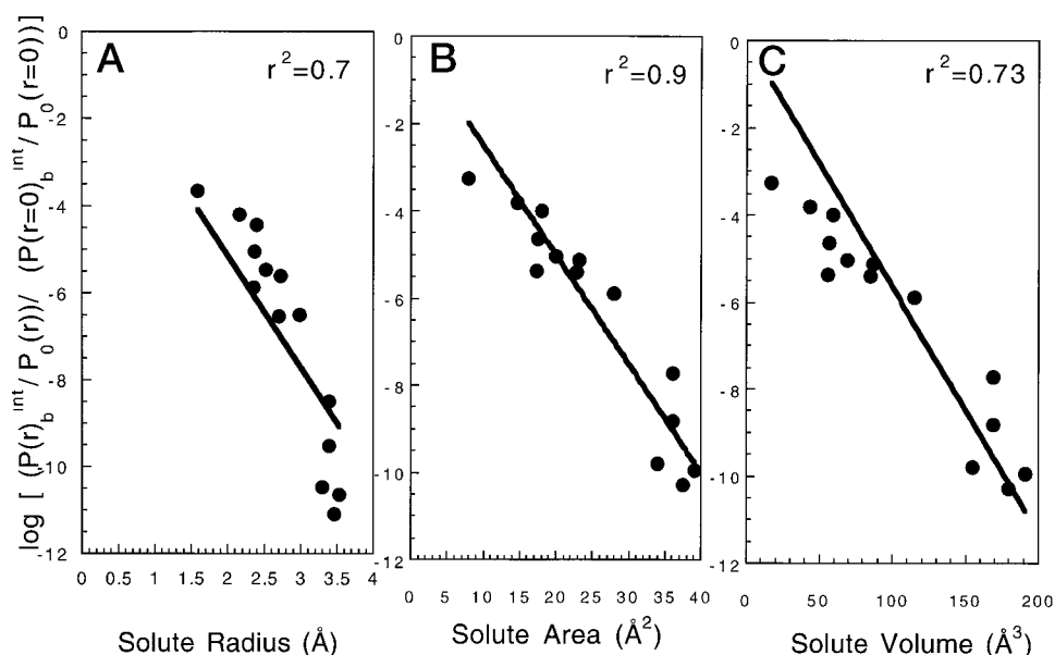
FIGURE 4 Replot of the experimental data shown in Figure 3 (normalized with respect to the solute permeability corresponding to a solute with r = 0 as predicted by Eq. 31, that is, [P_b^{\text{int}}(r)/P_0(r)]/[P_b^{\text{int}}(r = 0)/P_0(r = 0)] ) as a function of (A) solute radius, (B) cross-sectional area, and (C) volume. The solid lines correspond to exponential fits of the experimental data using the equation [P_b^{\text{int}}(r)/P_0(r)]/[P_b^{\text{int}}(r = 0)/P_0(r = 0)] = \exp(-\alpha G) , where G is either solute radius, cross-sectional area, or volume.
